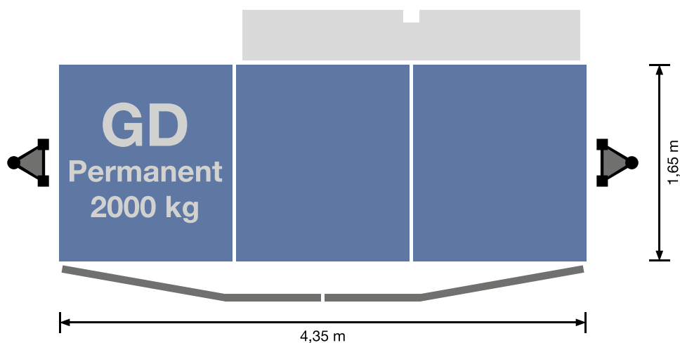
GEDA 1500 ZP P platform GD-Permanent 2 loading doors / 1 unloading double ramp
